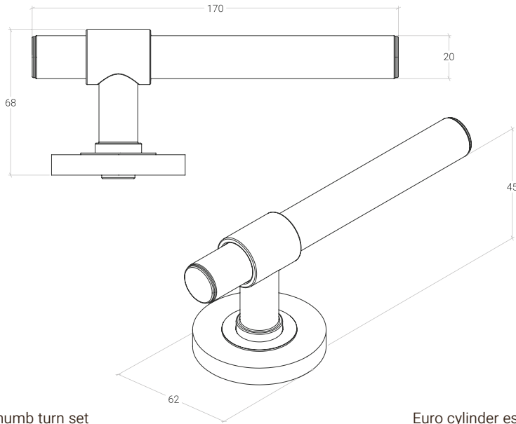
Privacy thumb turn set
