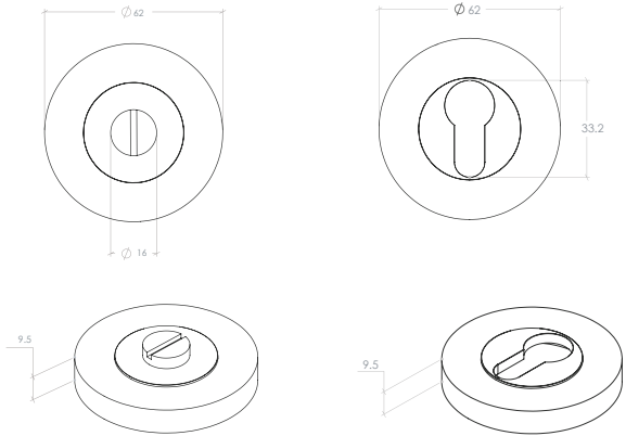
Euro cylinder escutcheon set
