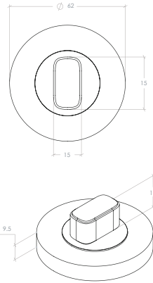
Privacy thumb turn set
