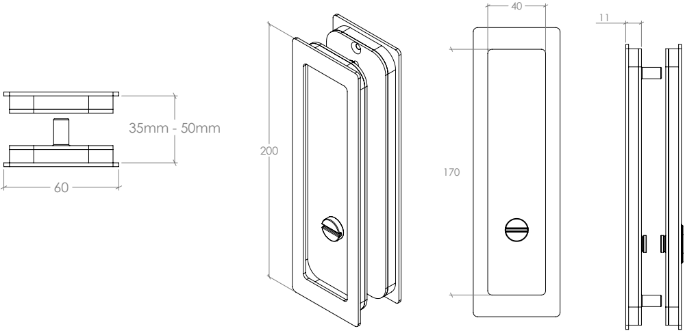
Cavity Slider With Lock
