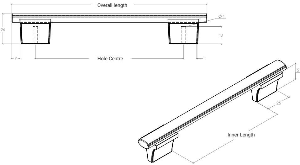
D Handle
