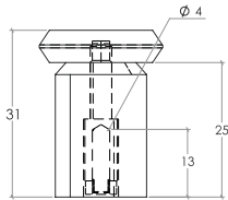
Round Knob
