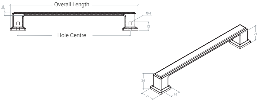
D Handle
