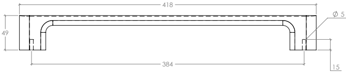
D Handle
