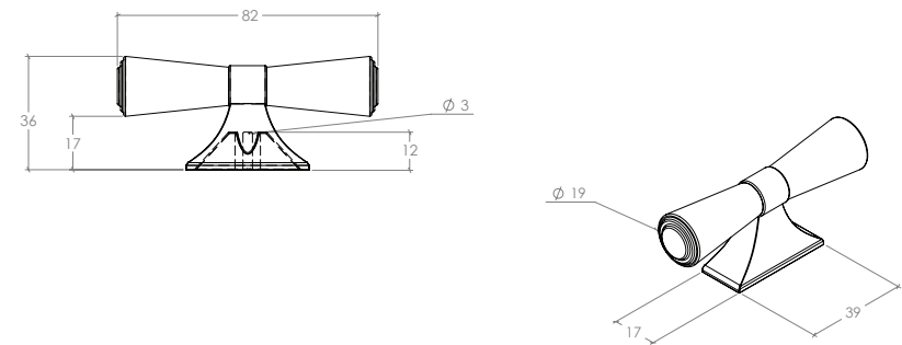
Bar Handle
